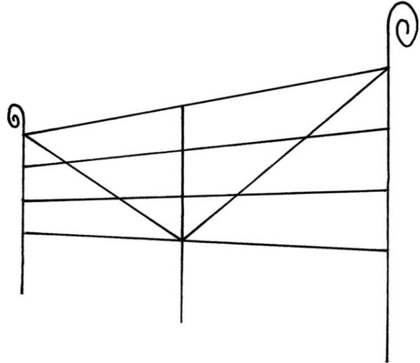
Grande Plant Gates 100cm wide 38cm tall (above ground, not including scrolls) Sold in Pairs (made from heavier duty wire)
